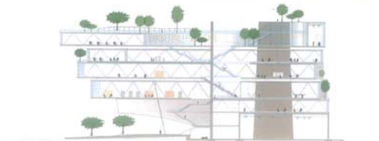
SECTION SECTION, North View, scale 1:100
